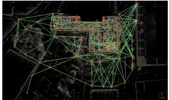
Plan view of laser scan locations, Boston, MA
